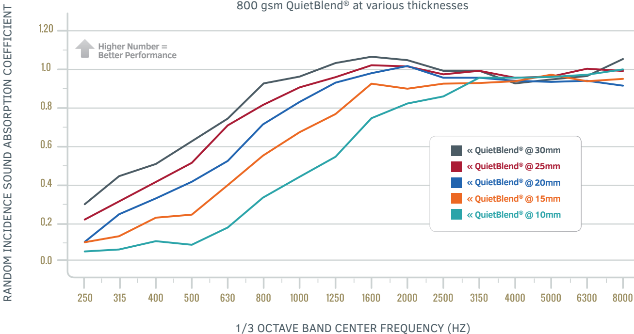
Random Incidence Sound Absorption 800 gsm QuietBlend® at various thicknesses
